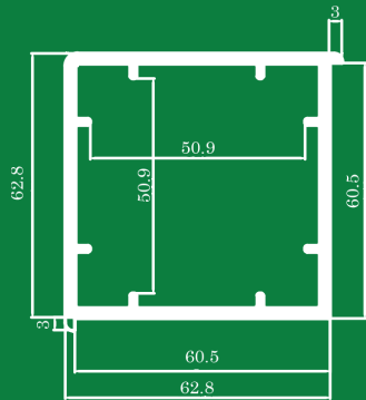
90 DEGREE CORNER CP90C 0.965 kg/m
