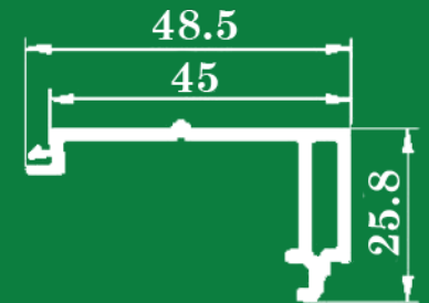
JALOUSIE WINDOW HOLDER BK60 0.26 kg/m
