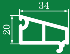
CASEMENT SINGLE GLASS BEAD GB34 0.29 kg/m
