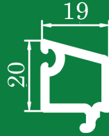
CASEMENT DOUBLE GLASS BEAD GB19 0.215 kg/m
